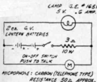
MODULATED LIGHT TRANSMITTER
